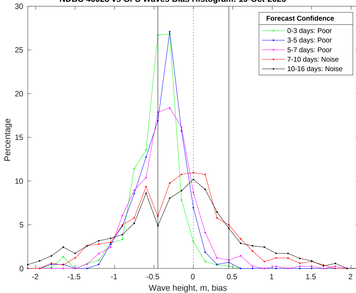
NDBC 46028 vs GFS Waves Bias Histogram: 19-Oct-2025
