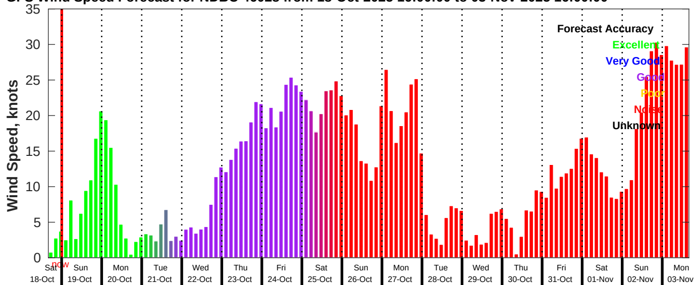
GFS Wind Speed Forecast for NDBC 46028 from 18-Oct-2025 16:00:00 to 03-Nov-2025 16:00:00
