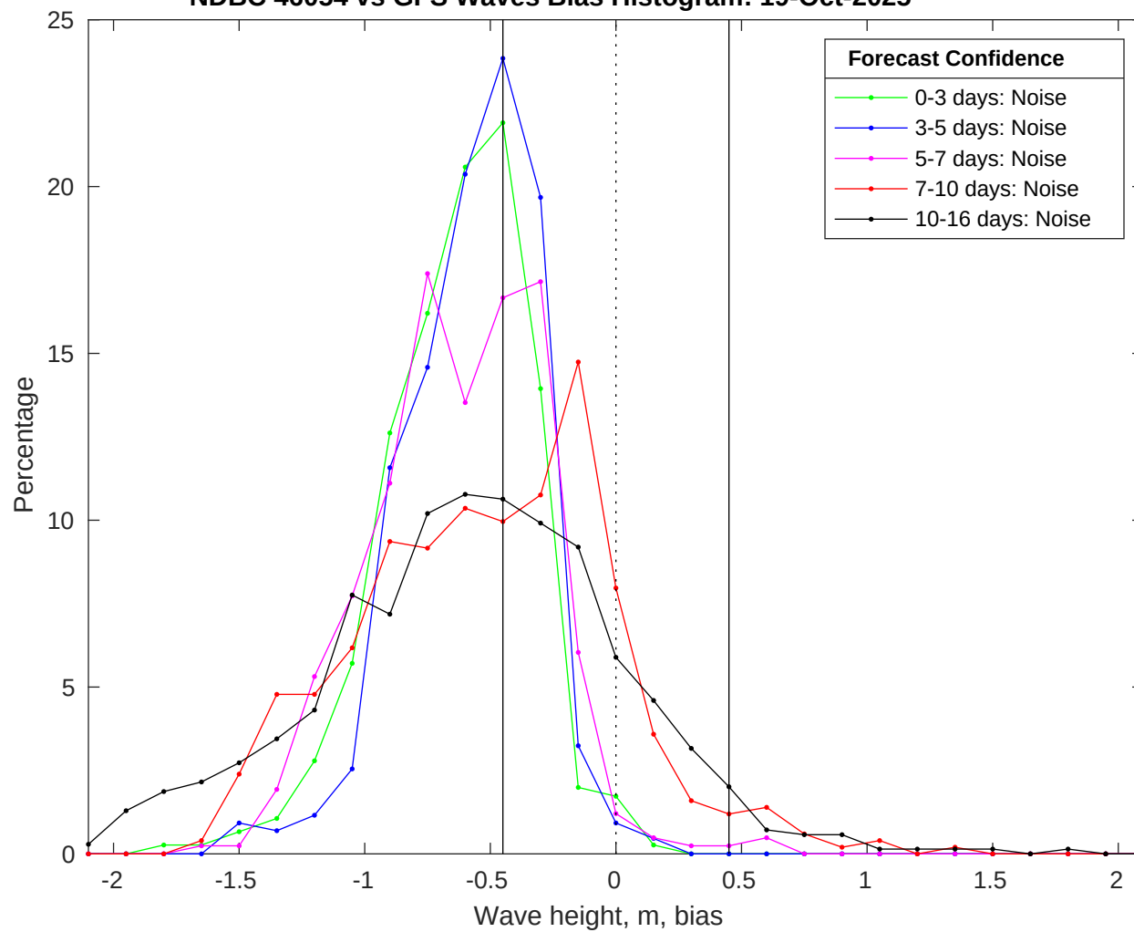
NDBC 46054 vs GFS Waves Bias Histogram: 19-Oct-2025
