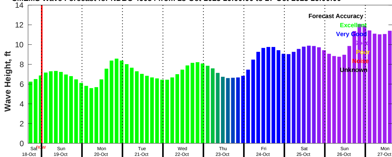
CMEMS Wave Forecast for NDBC 46054 from 18-Oct-2025 16:00:00 to 27-Oct-2025 16:00:00
