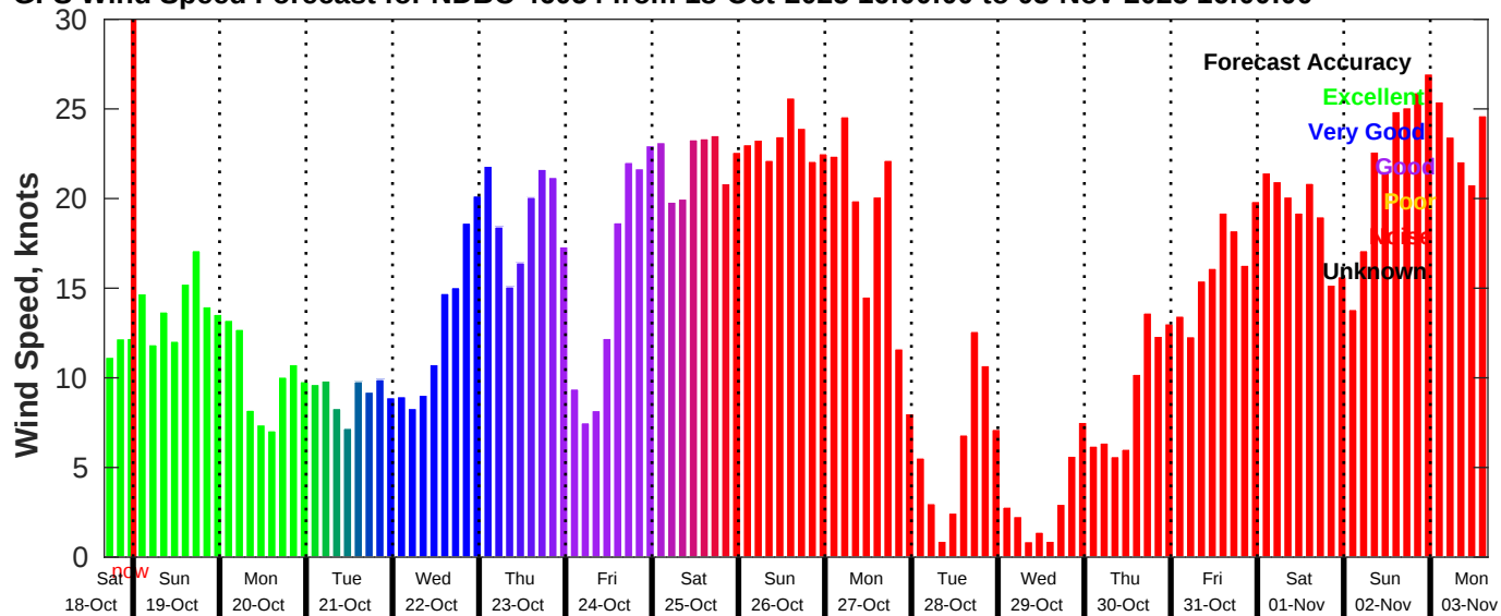
GFS Wind Speed Forecast for NDBC 46054 from 18-Oct-2025 16:00:00 to 03-Nov-2025 16:00:00
