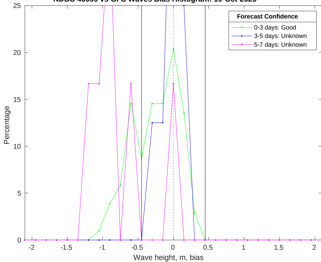
NDBC 46059 vs GFS Waves Bias Histogram: 19-Oct-2025
