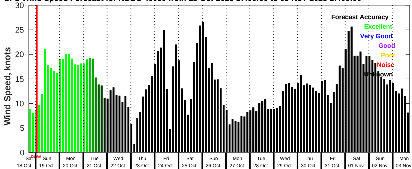
GFS Wind Speed Forecast for NDBC 46059 from 18-Oct-2025 17:00:00 to 03-Nov-2025 17:00:00
