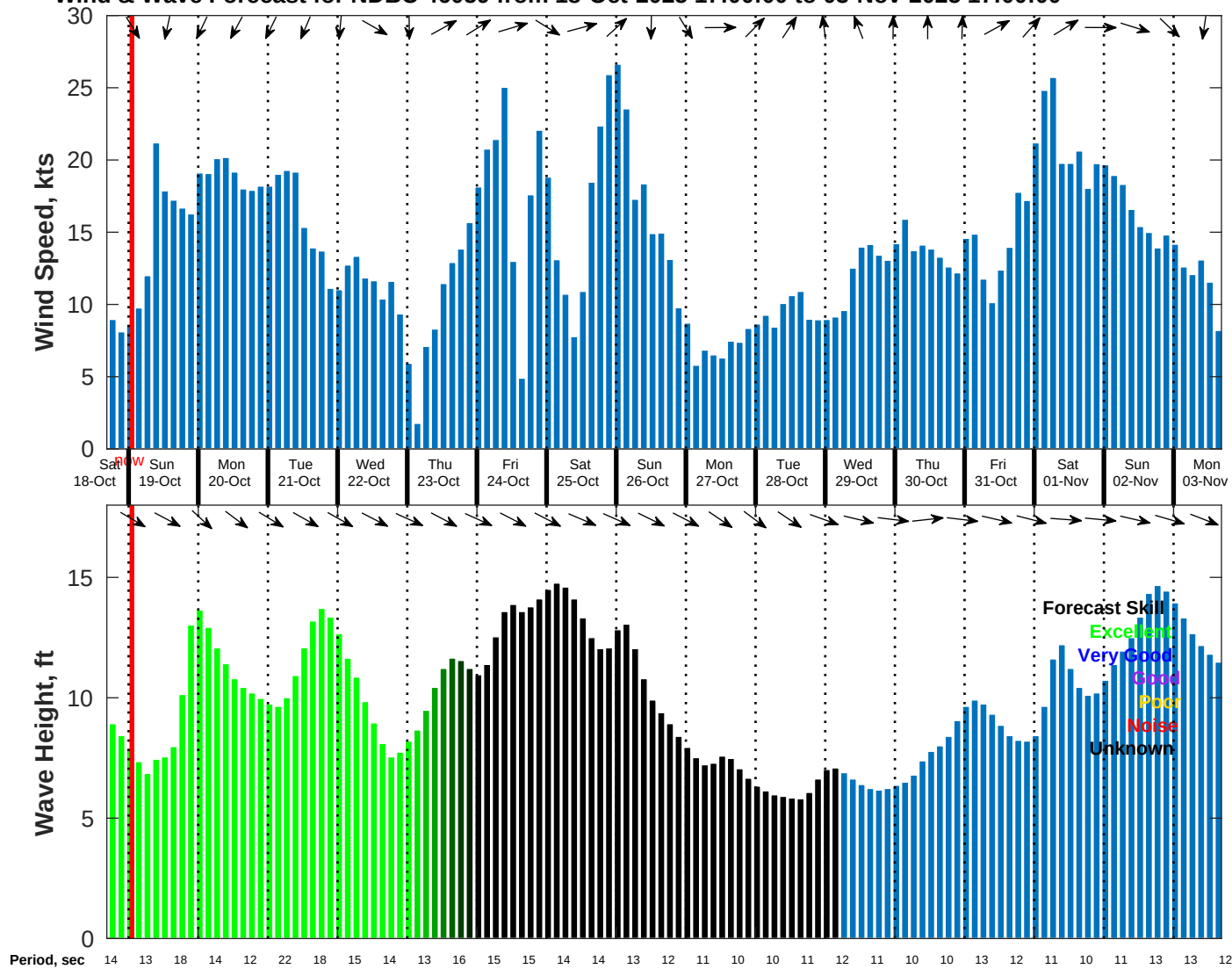
Wind & Wave Forecast for NDBC 46059 from 18-Oct-2025 17:00:00 to 03-Nov-2025 17:00:00
