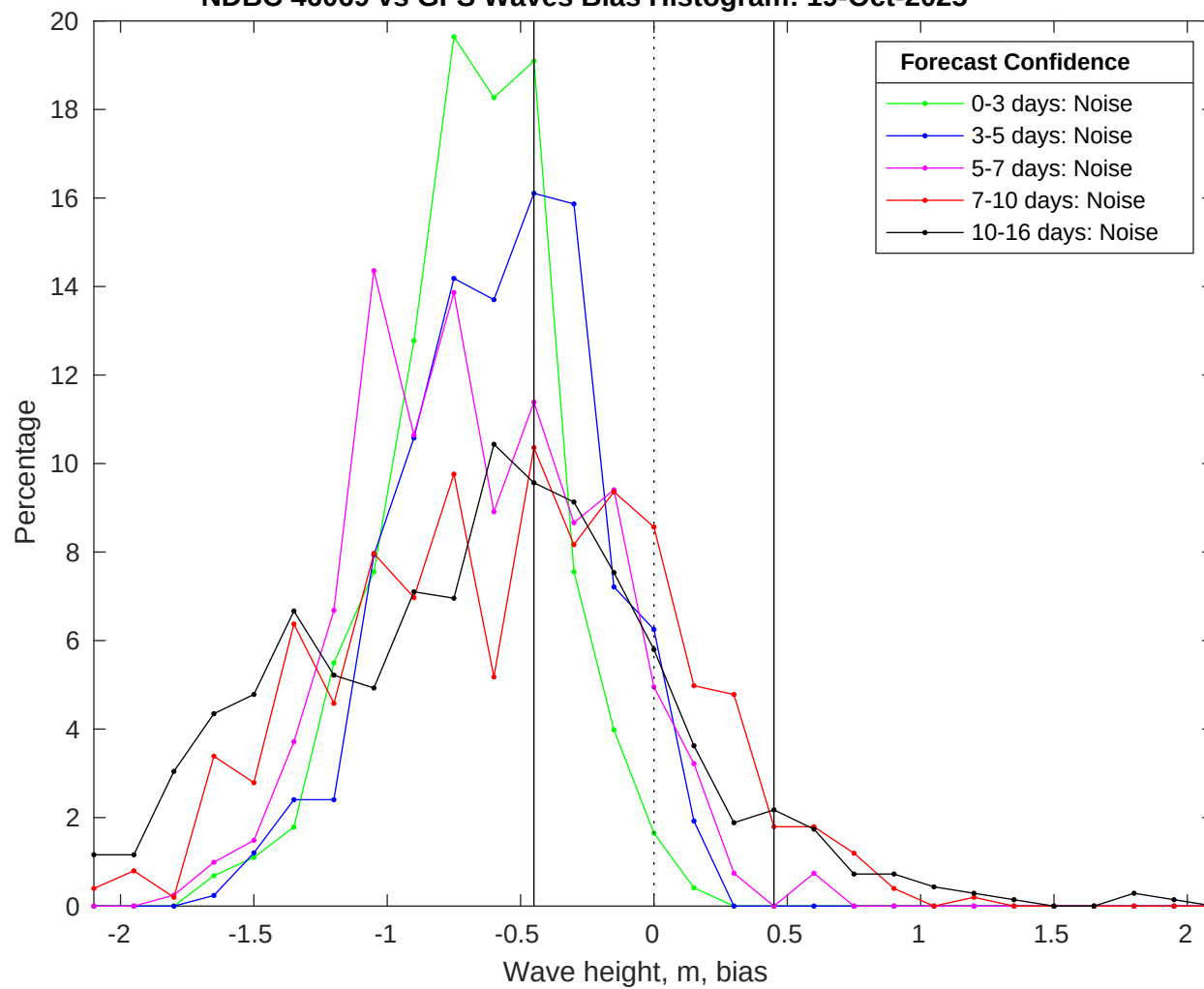
NDBC 46069 vs GFS Waves Bias Histogram: 19-Oct-2025
