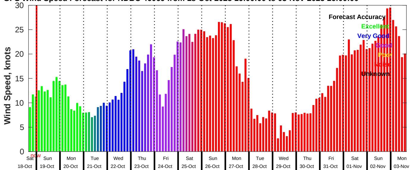
GFS Wind Speed Forecast for NDBC 46069 from 18-Oct-2025 16:00:00 to 03-Nov-2025 16:00:00
