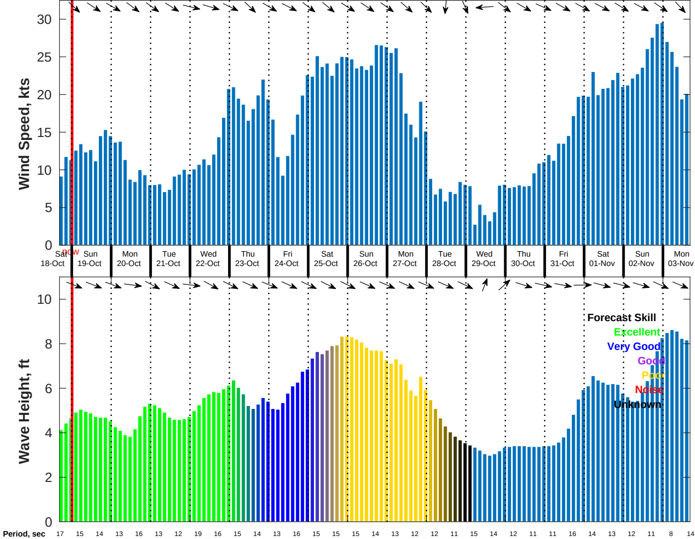
Wind & Wave Forecast for NDBC 46069 from 18-Oct-2025 16:00:00 to 03-Nov-2025 16:00:00
