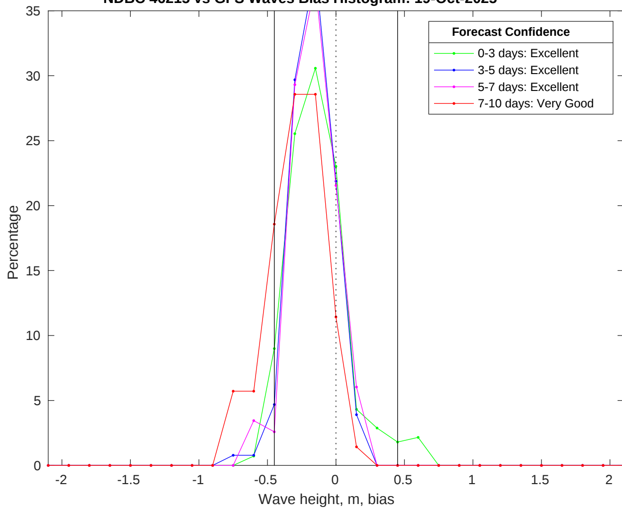
NDBC 46215 vs GFS Waves Bias Histogram: 19-Oct-2025
