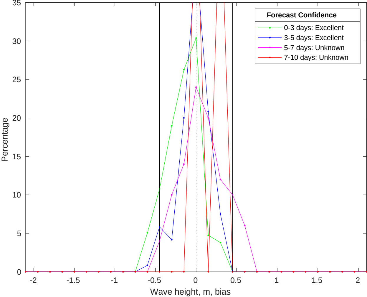
NDBC 46259 vs CMEMS Waves Bias Histogram: 19-Oct-2025
