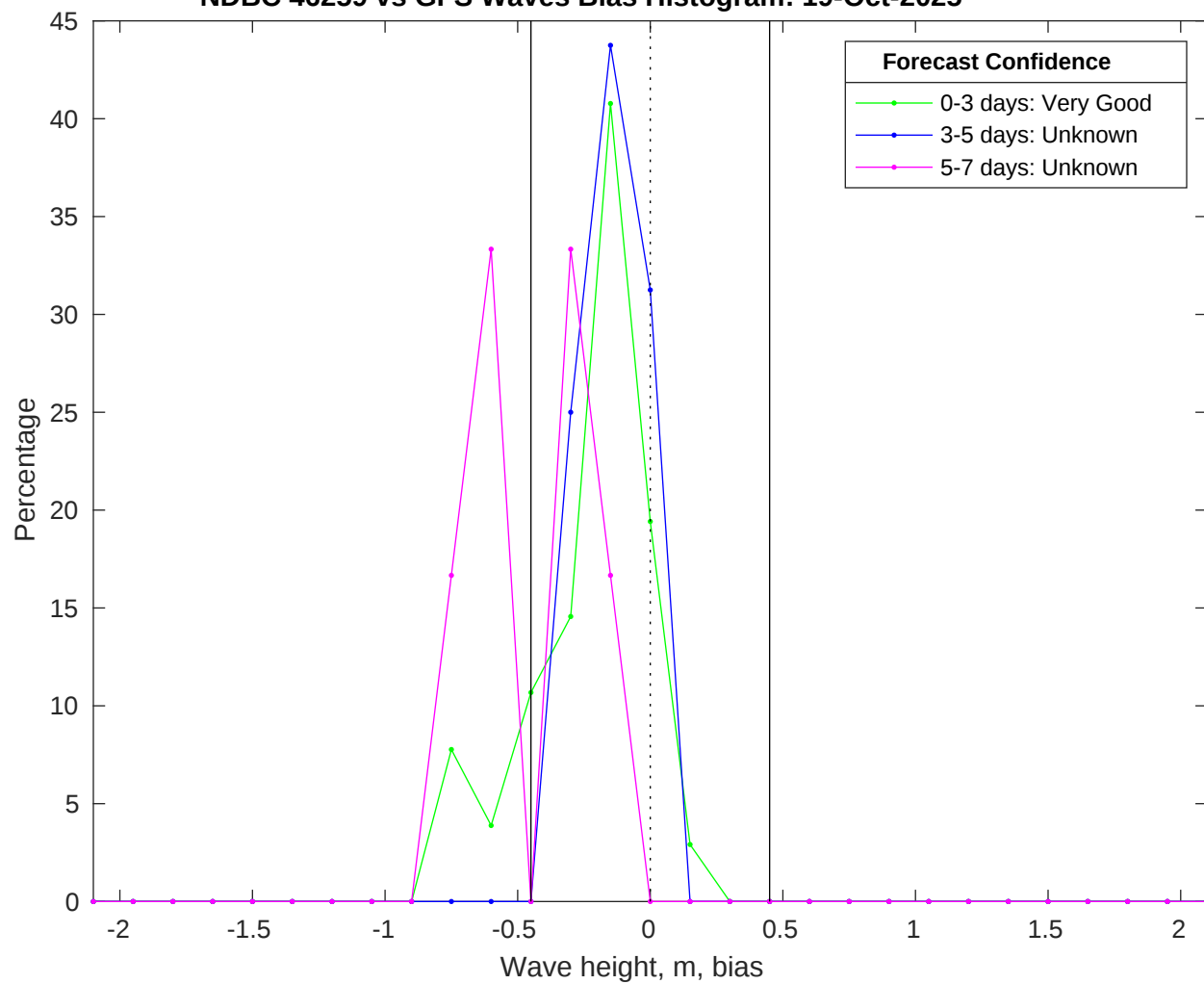
NDBC 46259 vs GFS Waves Bias Histogram: 19-Oct-2025
