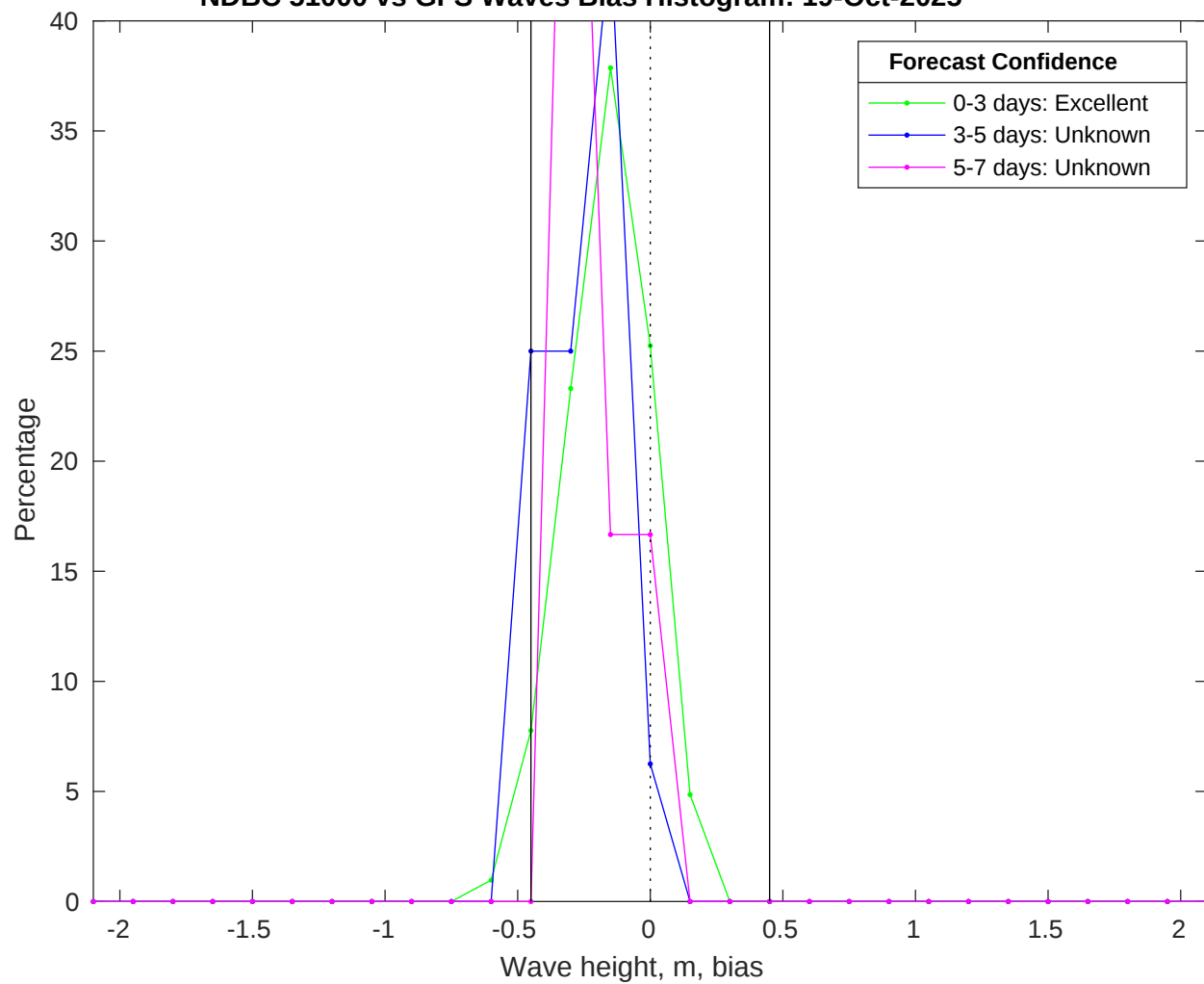
NDBC 51000 vs GFS Waves Bias Histogram: 19-Oct-2025
