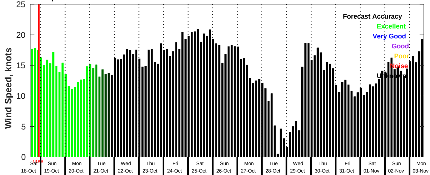
GFS Wind Speed Forecast for NDBC 51000 from 18-Oct-2025 14:00:00 to 03-Nov-2025 14:00:00
