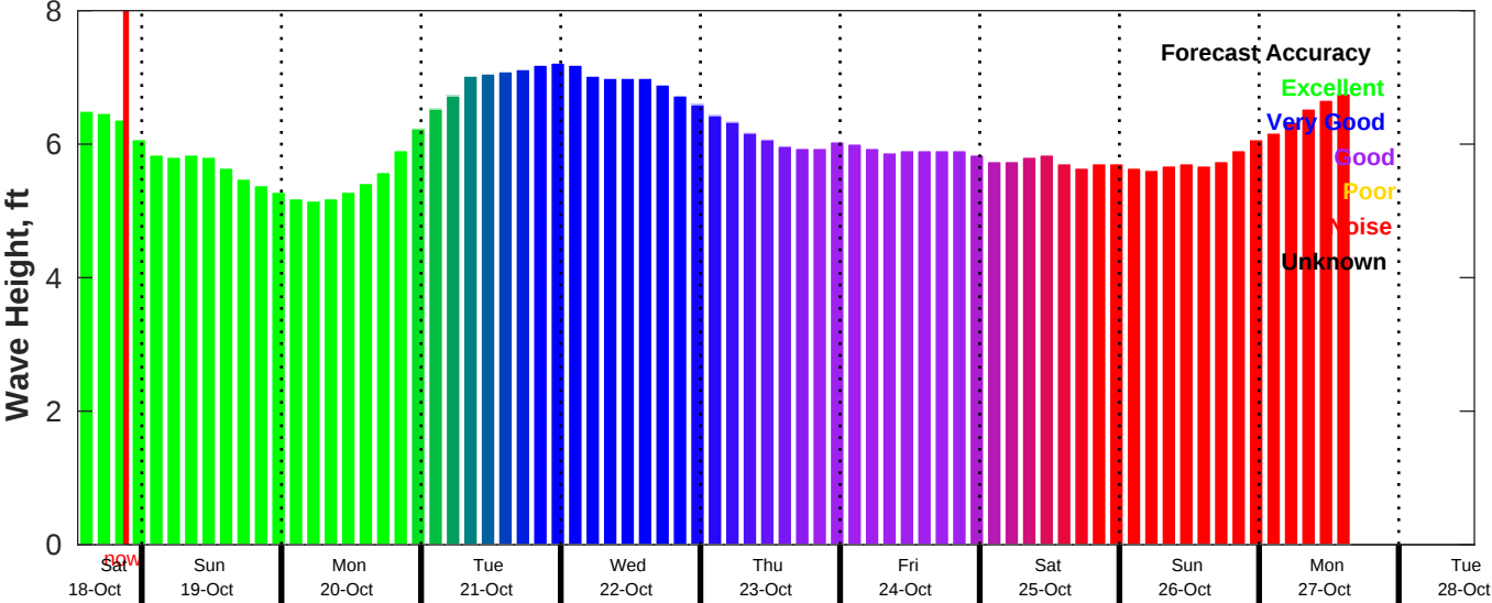
CMEMS Wave Forecast for NDBC 51209 from 18-Oct-2025 13:00:00 to 28-Oct-2025 13:00:00
