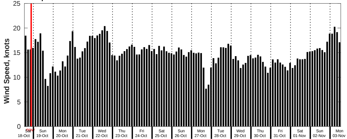
GFS Wind Speed Forecast for NDBC 51209 from 18-Oct-2025 13:00:00 to 03-Nov-2025 13:00:00
