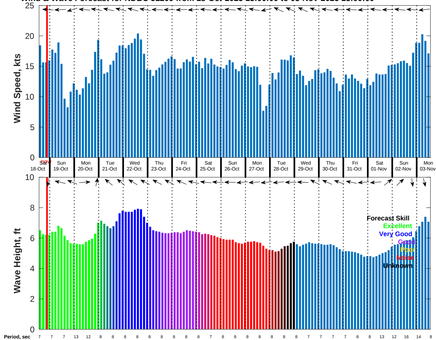
Wind & Wave Forecast for NDBC 51209 from 18-Oct-2025 13:00:00 to 03-Nov-2025 13:00:00
