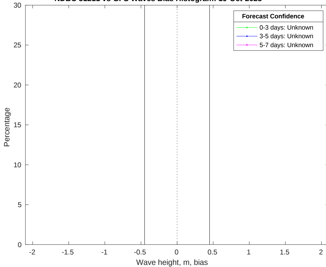
NDBC 51211 vs GFS Waves Bias Histogram: 19-Oct-2025
