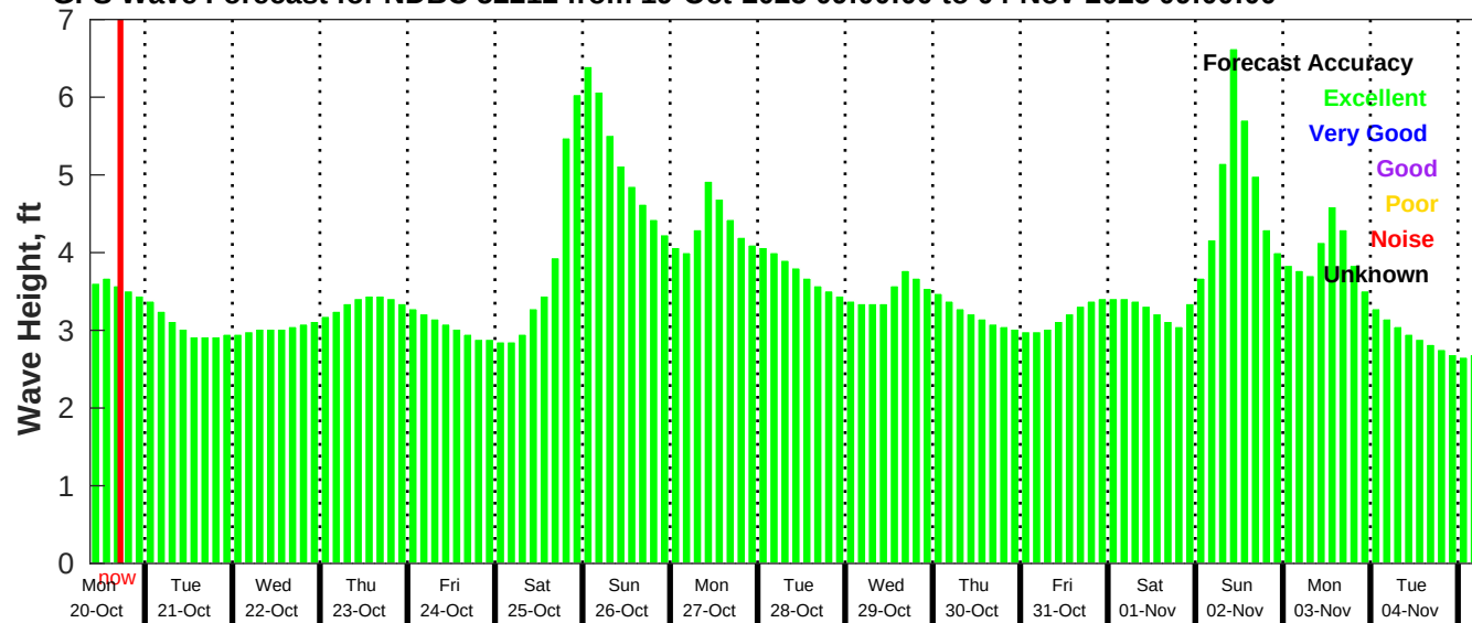
GFS Wave Forecast for NDBC 52212 from 19-Oct-2025 09:00:00 to 04-Nov-2025 09:00:00
