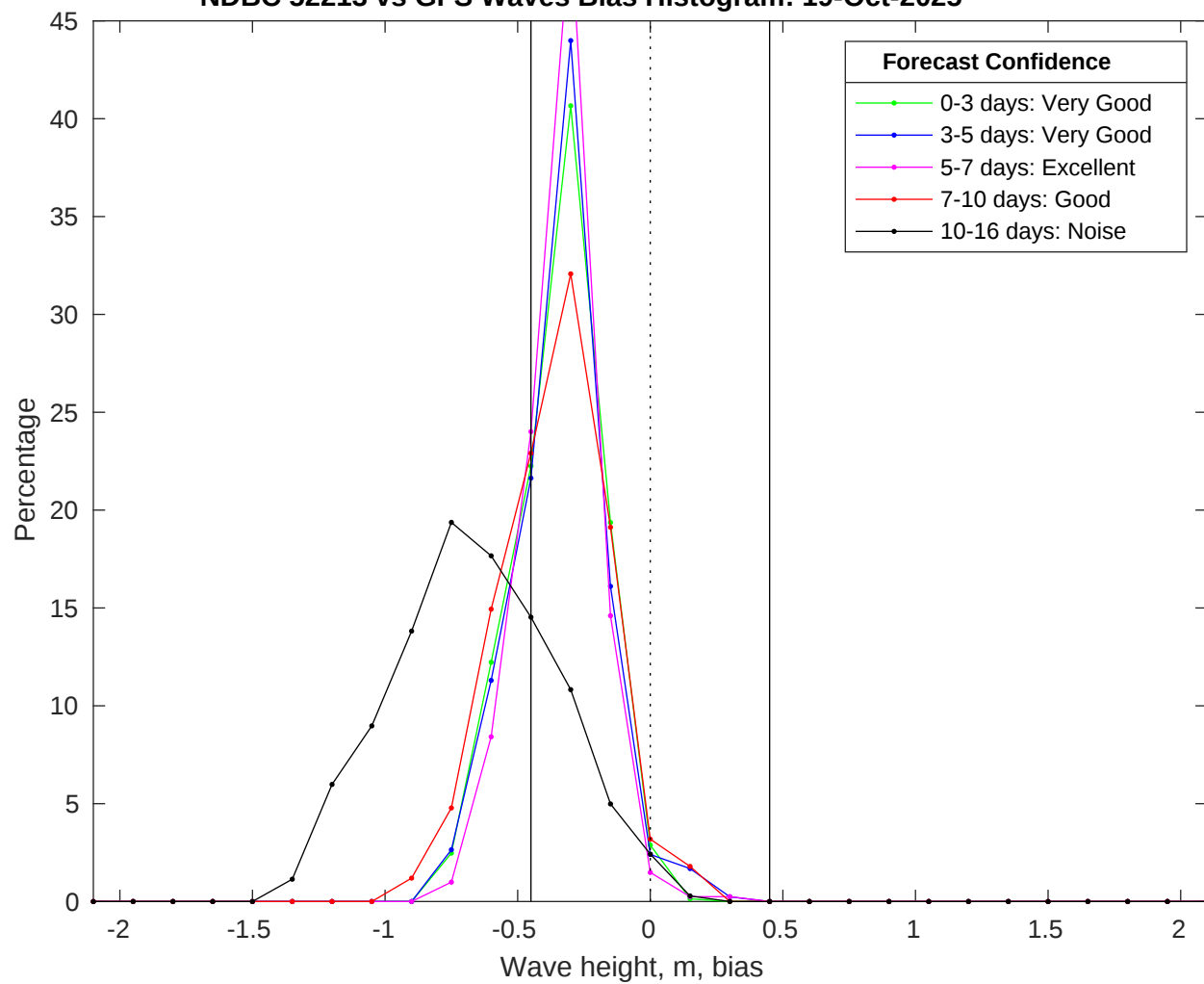
NDBC 52213 vs GFS Waves Bias Histogram: 19-Oct-2025
