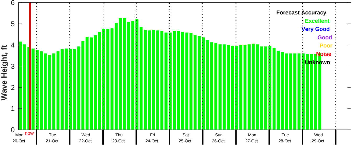
CMEMS Wave Forecast for NDBC 52213 from 19-Oct-2025 11:00:00 to 29-Oct-2025 11:00:00
