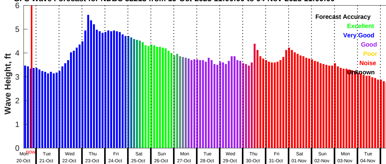
GFS Wave Forecast for NDBC 52213 from 19-Oct-2025 11:00:00 to 04-Nov-2025 11:00:00
