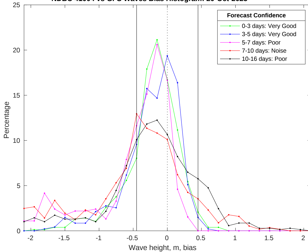
NDBC 41004 vs GFS Waves Bias Histogram: 20-Oct-2025
