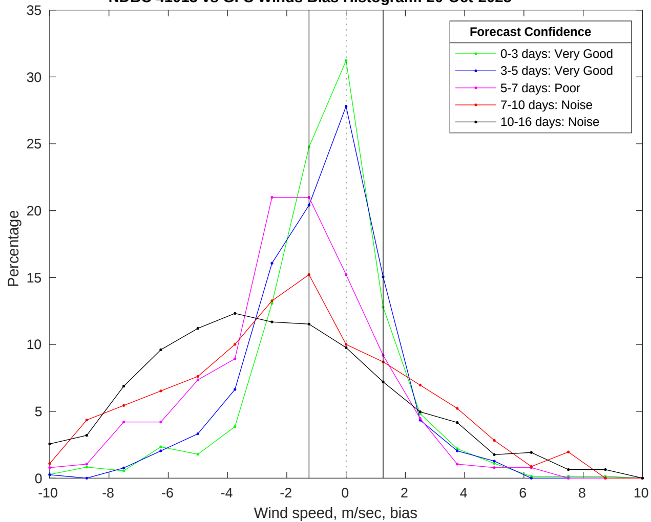
NDBC 41013 vs GFS Winds Bias Histogram: 20-Oct-2025
