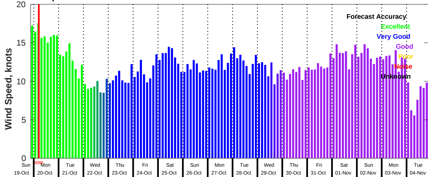
GFS Wind Speed Forecast for NDBC 41040 from 19-Oct-2025 21:00:00 to 04-Nov-2025 21:00:00
