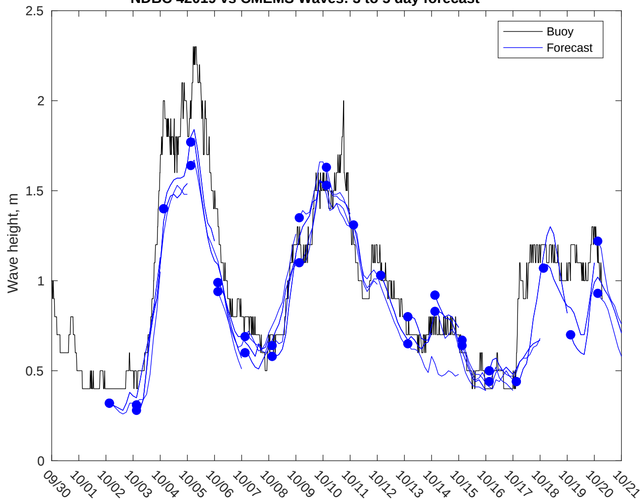
NDBC 42019 vs CMEMS Waves: 3 to 5 day forecast
