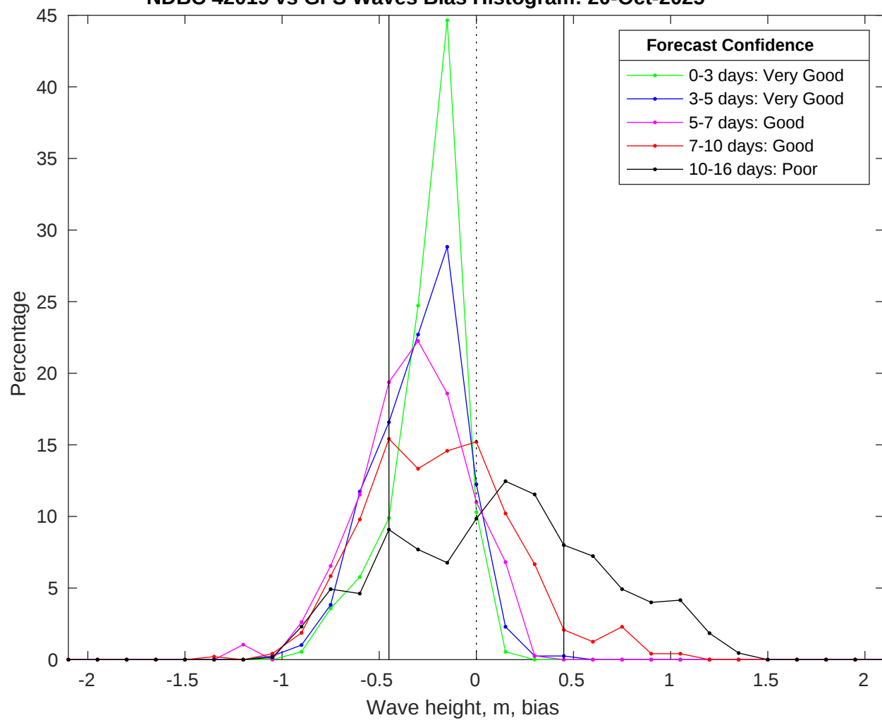
NDBC 42019 vs GFS Waves Bias Histogram: 20-Oct-2025
