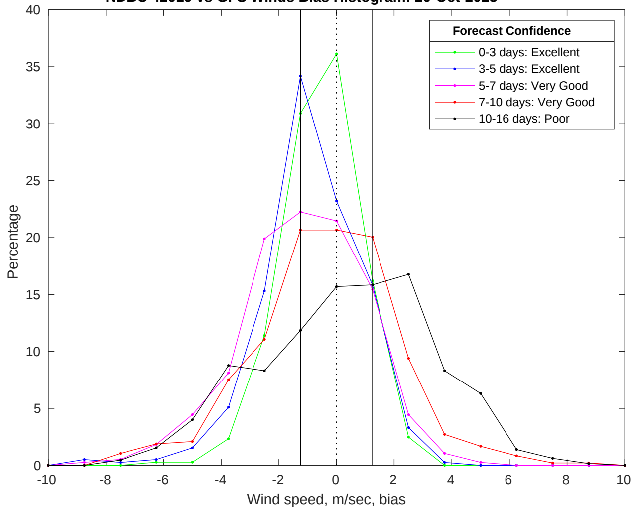
NDBC 42019 vs GFS Winds Bias Histogram: 20-Oct-2025
