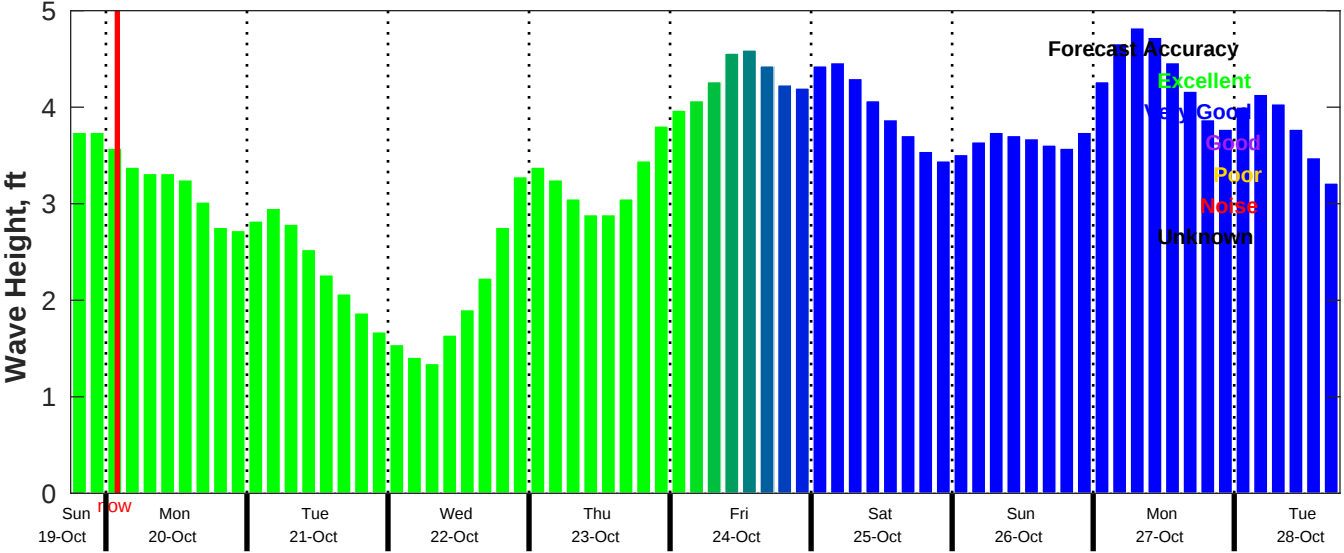
CMEMS Wave Forecast for NDBC 42019 from 19-Oct-2025 18:00:00 to 28-Oct-2025 18:00:00
