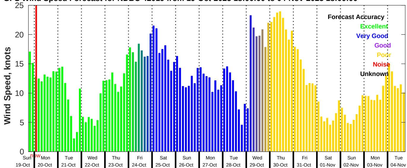
GFS Wind Speed Forecast for NDBC 42019 from 19-Oct-2025 18:00:00 to 04-Nov-2025 18:00:00
