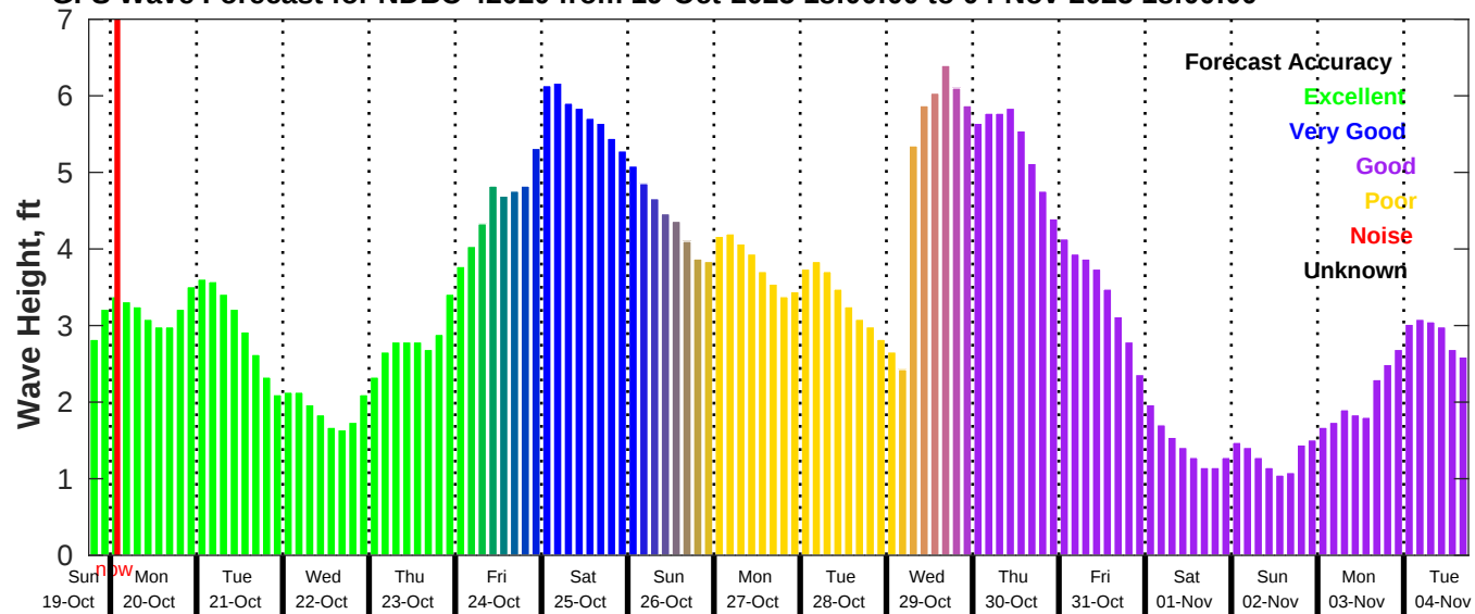
GFS Wave Forecast for NDBC 42020 from 19-Oct-2025 18:00:00 to 04-Nov-2025 18:00:00
