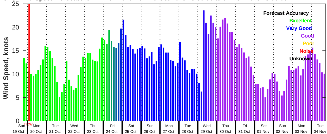
GFS Wind Speed Forecast for NDBC 42020 from 19-Oct-2025 18:00:00 to 04-Nov-2025 18:00:00
