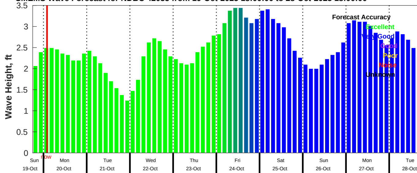
CMEMS Wave Forecast for NDBC 42035 from 19-Oct-2025 18:00:00 to 28-Oct-2025 18:00:00
