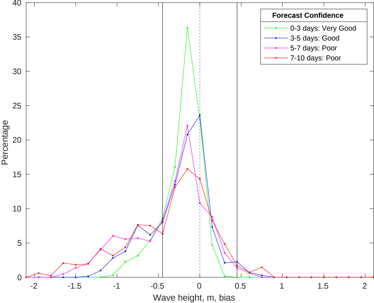
NDBC 42036 vs CMEMS Waves Bias Histogram: 20-Oct-2025
