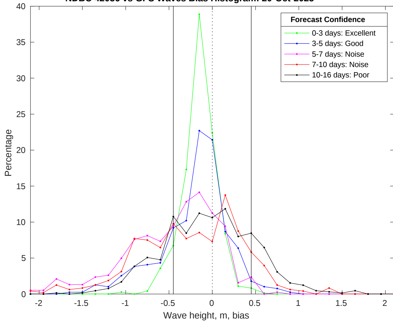
NDBC 42036 vs GFS Waves Bias Histogram: 20-Oct-2025
