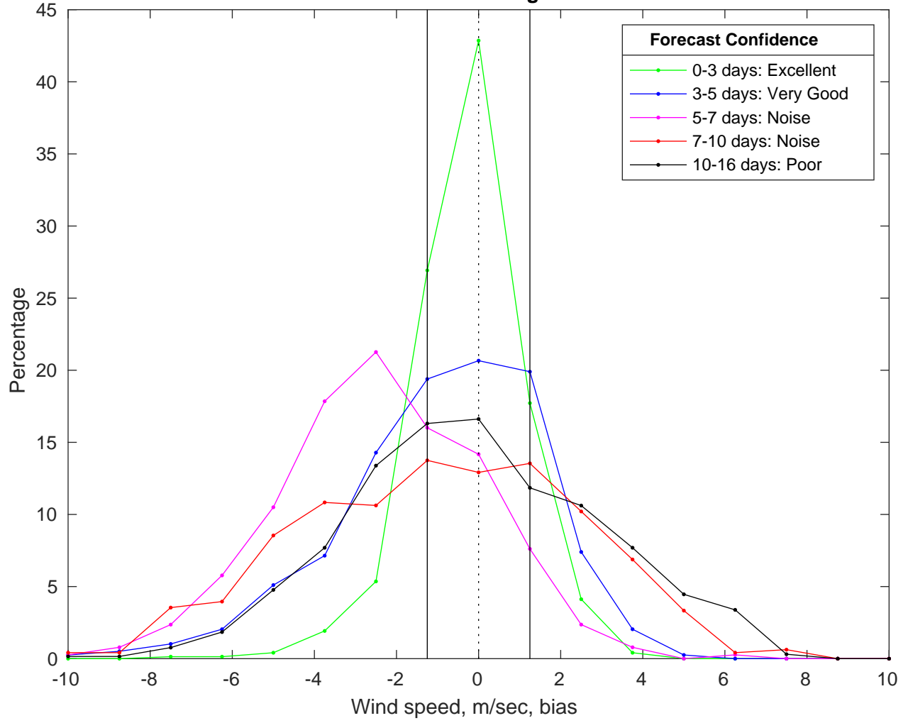
NDBC 42036 vs GFS Winds Bias Histogram: 20-Oct-2025
