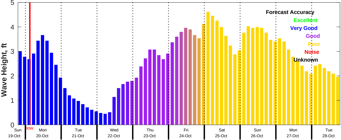
CMEMS Wave Forecast for NDBC 42036 from 19-Oct-2025 19:00:00 to 28-Oct-2025 19:00:00
