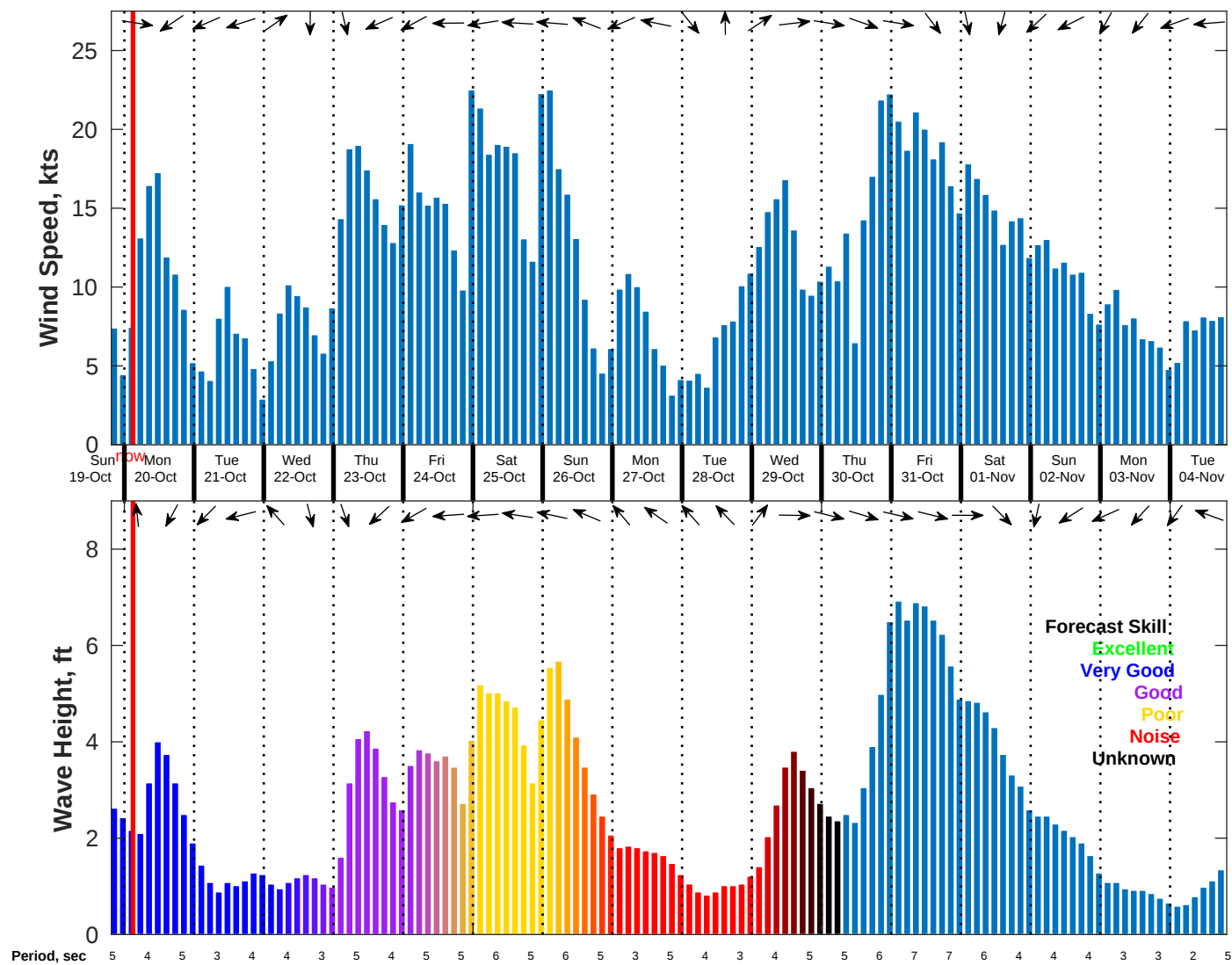
Wind & Wave Forecast for NDBC 42036 from 19-Oct-2025 19:00:00 to 04-Nov-2025 19:00:00
