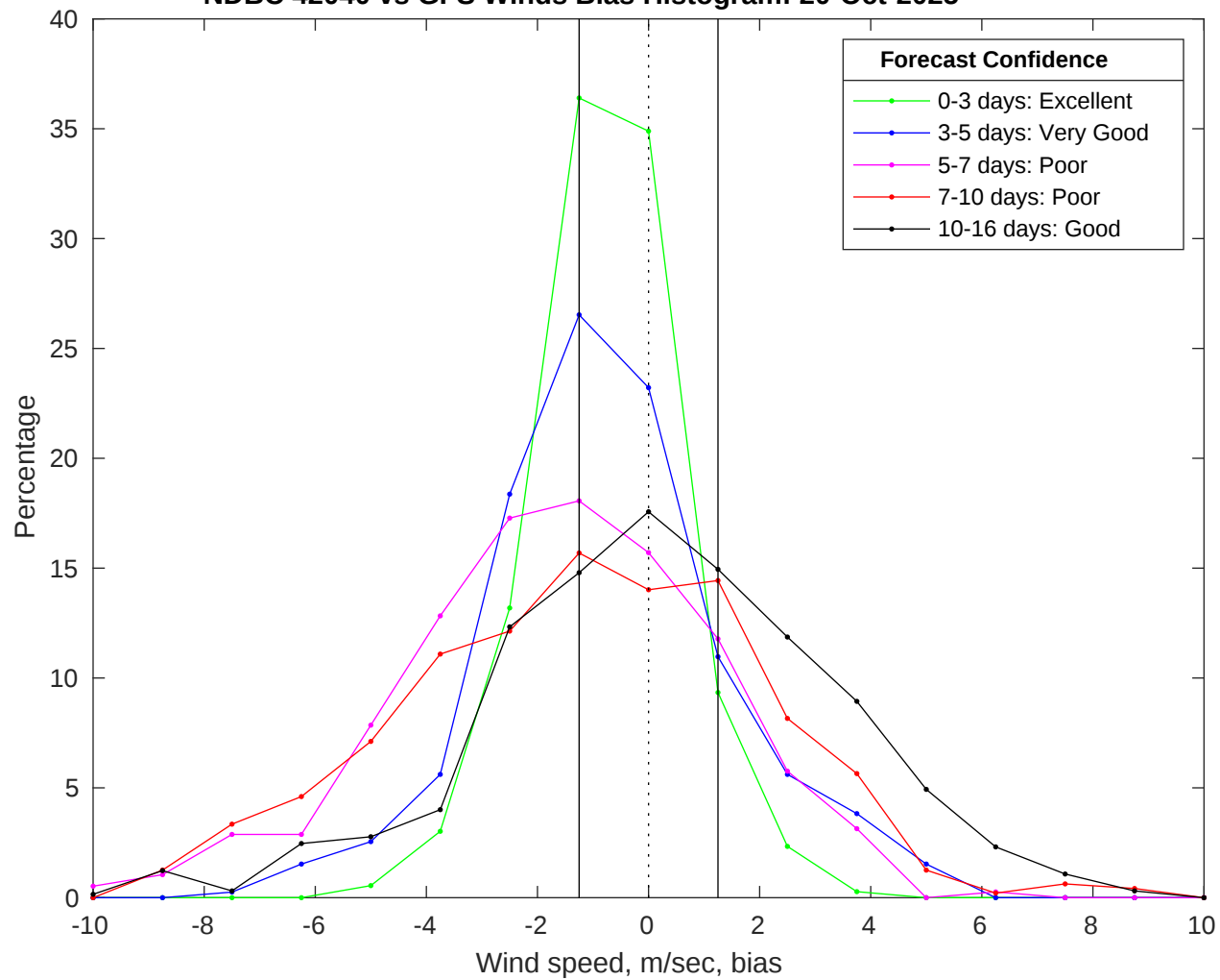
NDBC 42040 vs GFS Winds Bias Histogram: 20-Oct-2025
