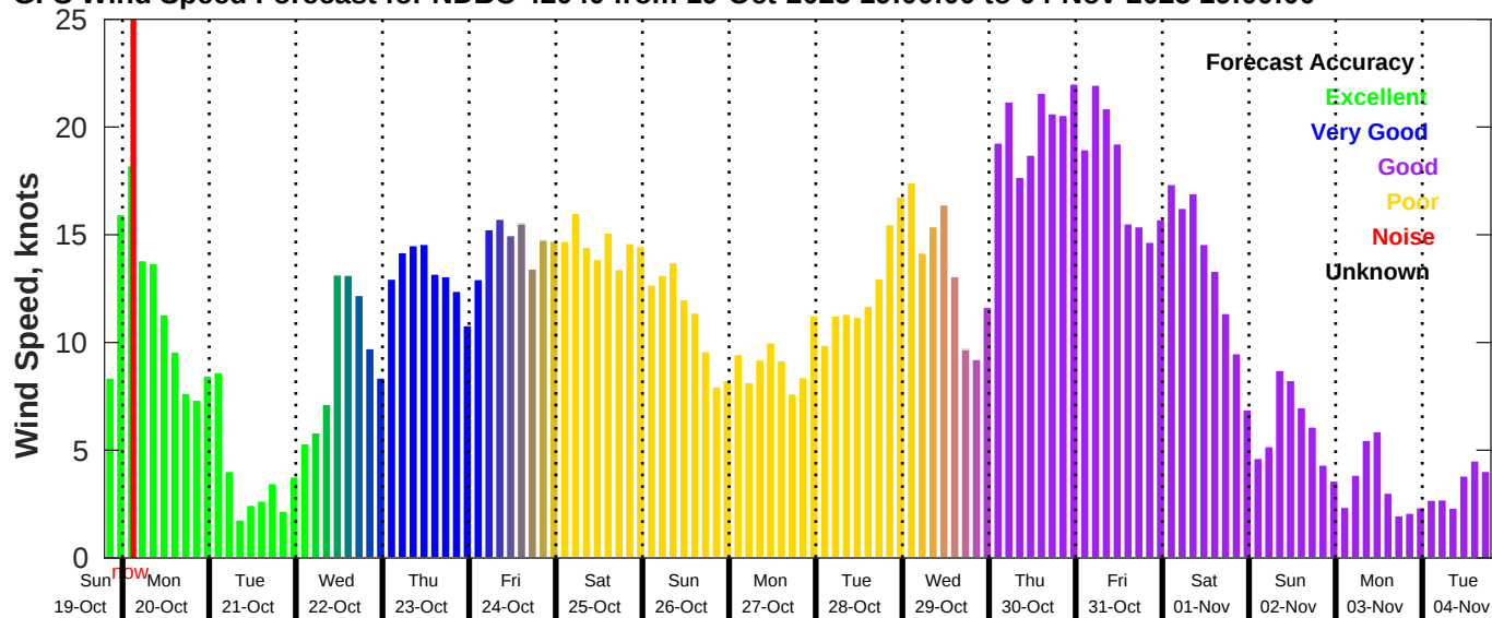
GFS Wind Speed Forecast for NDBC 42040 from 19-Oct-2025 19:00:00 to 04-Nov-2025 19:00:00
