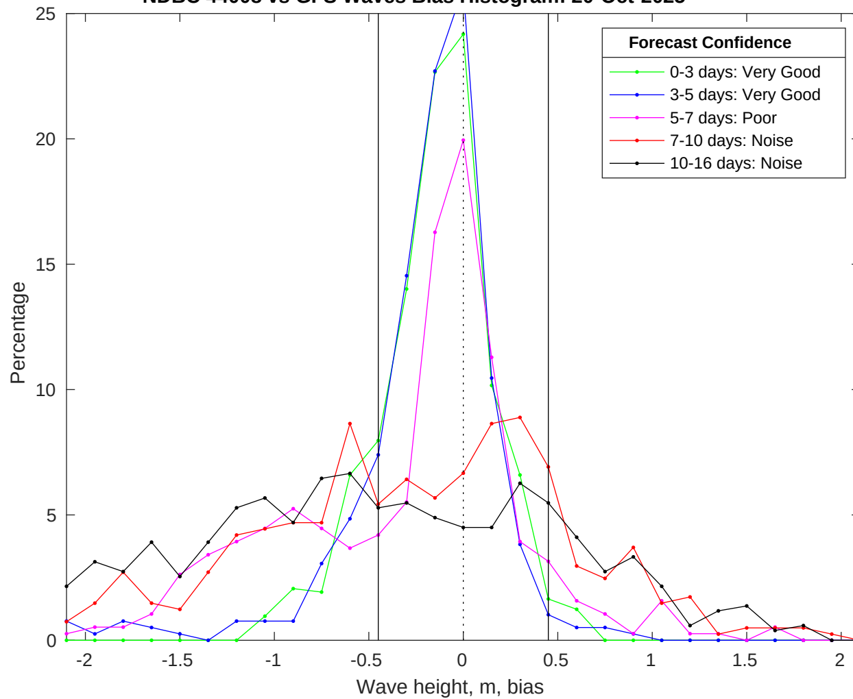
NDBC 44008 vs GFS Waves Bias Histogram: 20-Oct-2025
