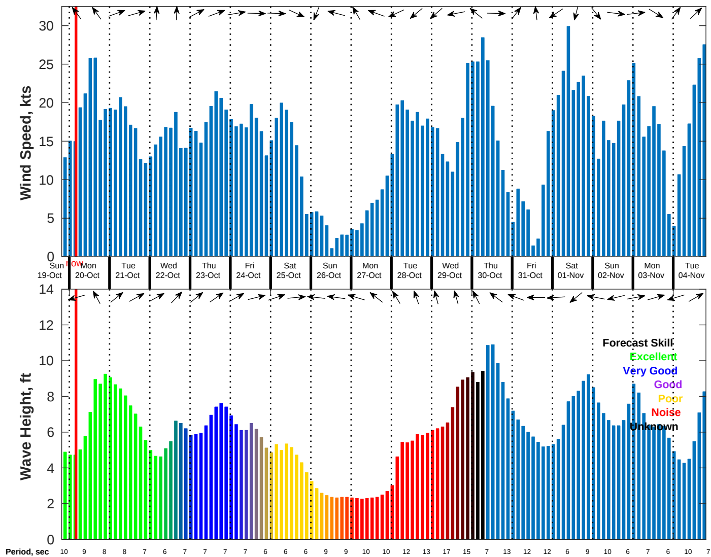
Wind & Wave Forecast for NDBC 44008 from 19-Oct-2025 20:00:00 to 04-Nov-2025 20:00:00
