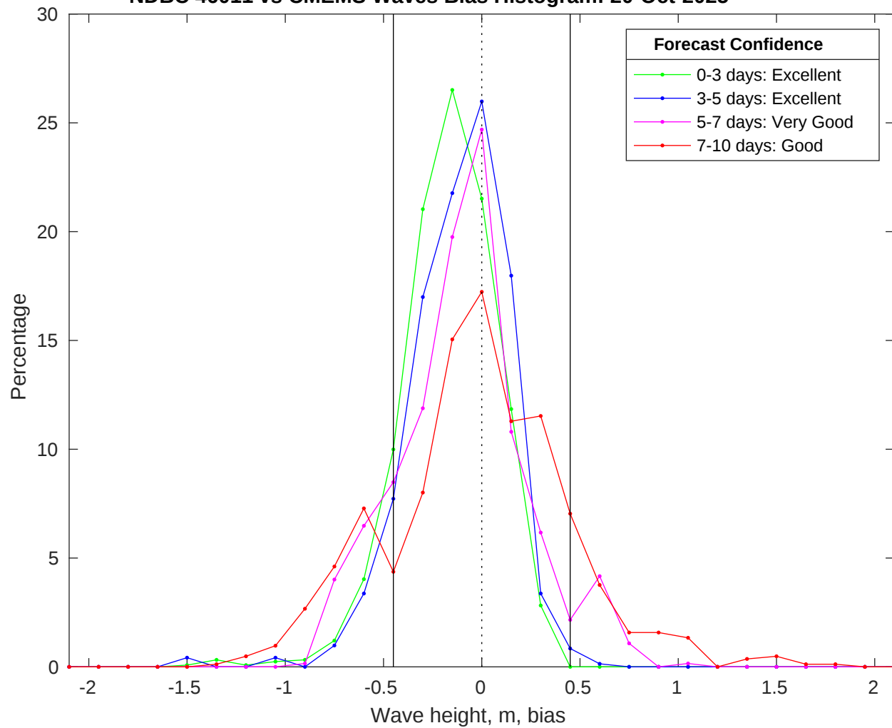
NDBC 46011 vs CMEMS Waves Bias Histogram: 20-Oct-2025
