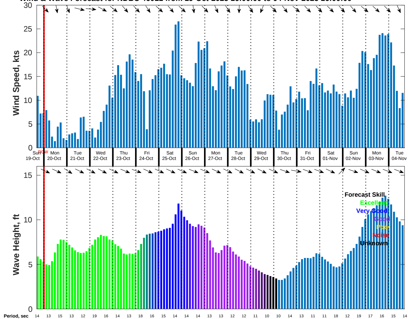
Wind & Wave Forecast for NDBC 46011 from 19-Oct-2025 16:00:00 to 04-Nov-2025 16:00:00
