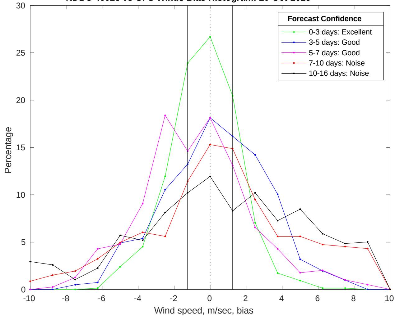
NDBC 46028 vs GFS Winds Bias Histogram: 20-Oct-2025
