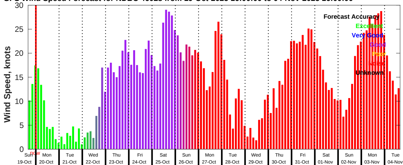
GFS Wind Speed Forecast for NDBC 46028 from 19-Oct-2025 16:00:00 to 04-Nov-2025 16:00:00
