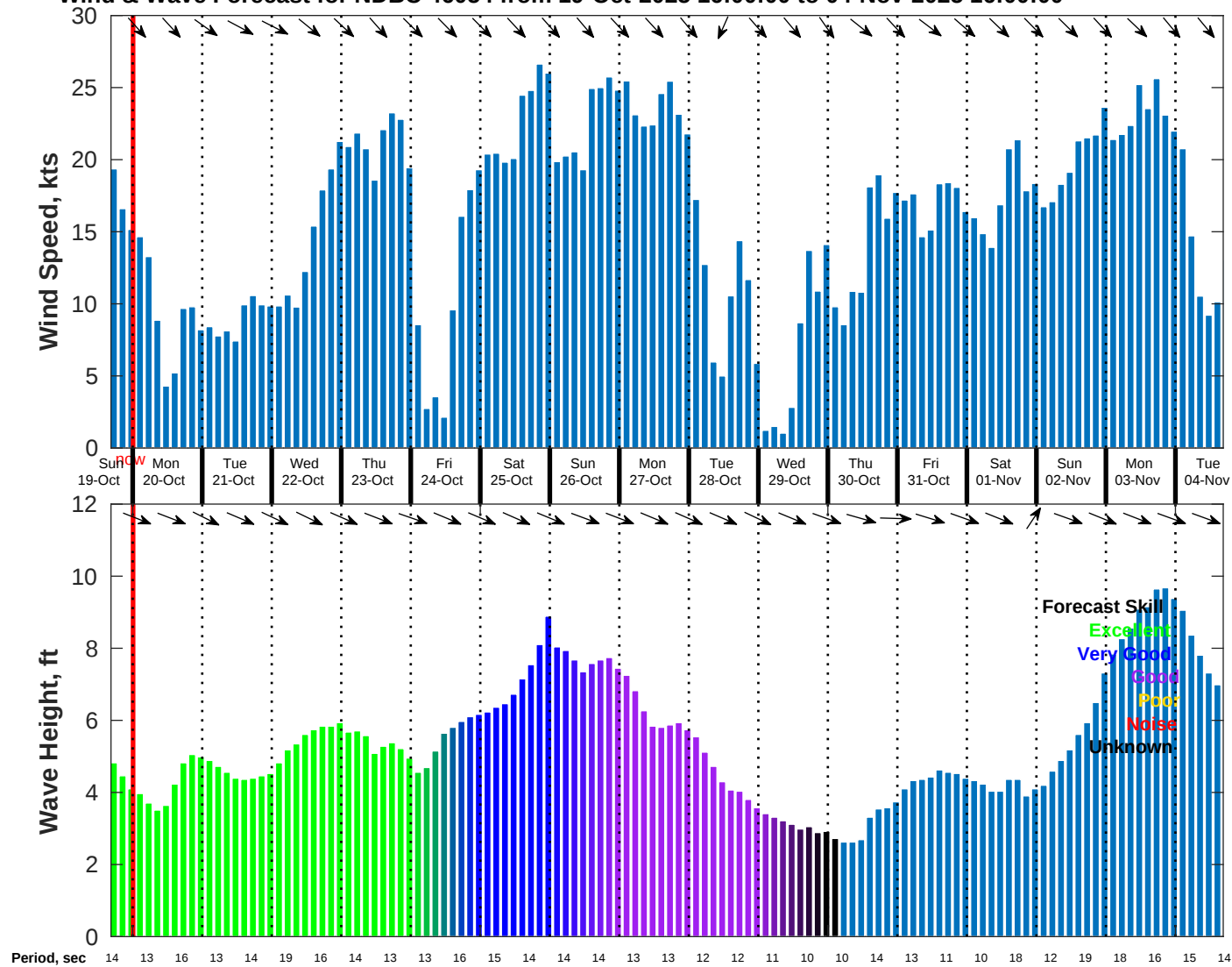
Wind & Wave Forecast for NDBC 46054 from 19-Oct-2025 16:00:00 to 04-Nov-2025 16:00:00
