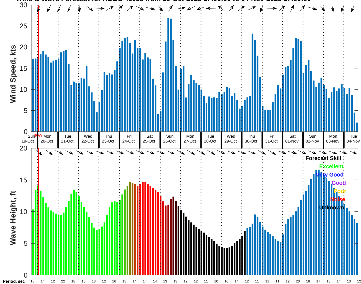
Wind & Wave Forecast for NDBC 46059 from 19-Oct-2025 17:00:00 to 04-Nov-2025 17:00:00
